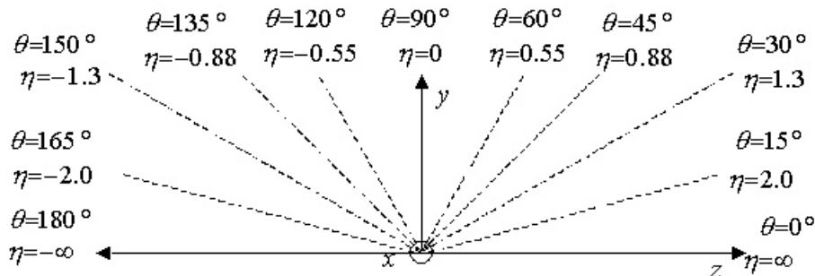
Figure 8: Corresponding values of \eta for different values of \theta
