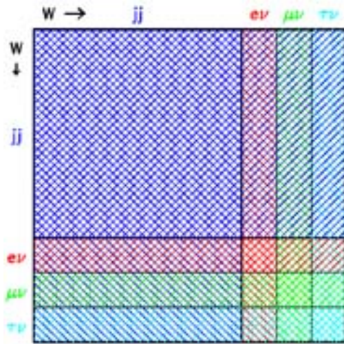
Figure 4: Top quark decay channels
