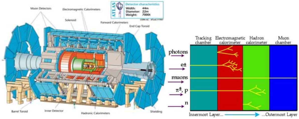
Figure 6: On the left the ATLAS detector and on the right a chart of the particle detecting capabilities of each subdetector
