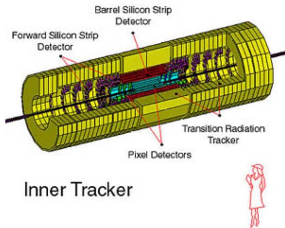
Figure 9: ATLAS' inner detector
