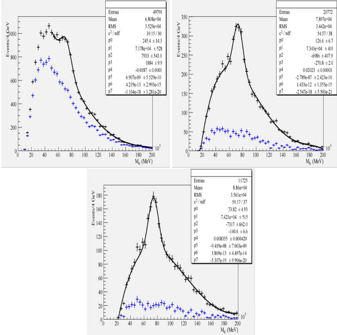
Figure 37: Invariant mass of the two light jets with a jet p_T cut of 20 GeV/c (left), 30 GeV/c (middle) and 40 GeV/c (right). Full histograms represent background distributions and hatched signal distributions.
