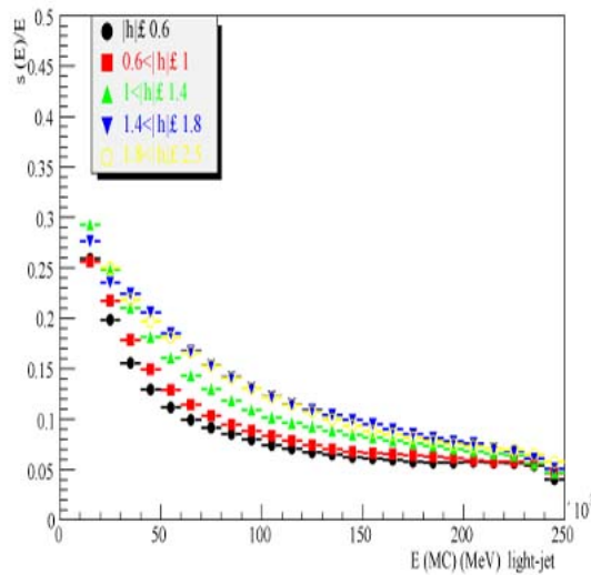
Figure 19: Energy jet resolution for different \eta ranges.
