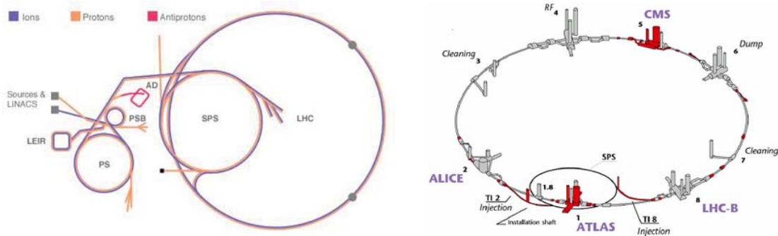
Figure 5: CERN's accelerator network
