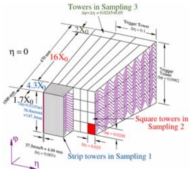
Figure 10: Granularity of the electromagnetic calorimeter
