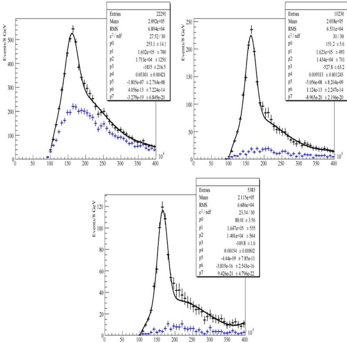
Figure 39: Invariant mass of the three jets with a jet p_T cut of 20 GeV/c (left), 30 GeV/c (middle) and 40 GeV/c (right) for those whose W reconstructed mass is between 50 and 90 GeV/ c^2 . Full histogram represents background distribution
