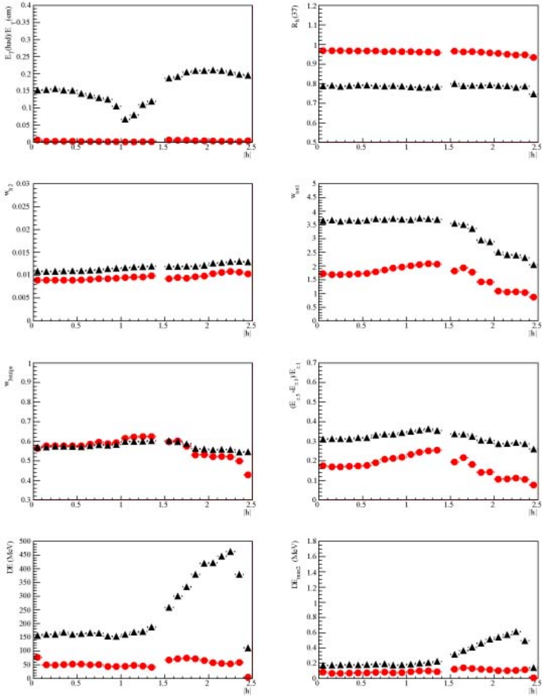
Figure 31: Distributions of the mean of each calorimetric discriminating variable as a function of the pseudo-rapidity |\eta| for electrons (circle) and jets (triangle).
