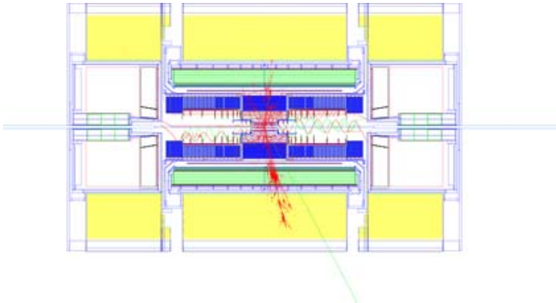
Figure 2: t\bar{t} event simulation inside the inner detector and the calorimeter.
