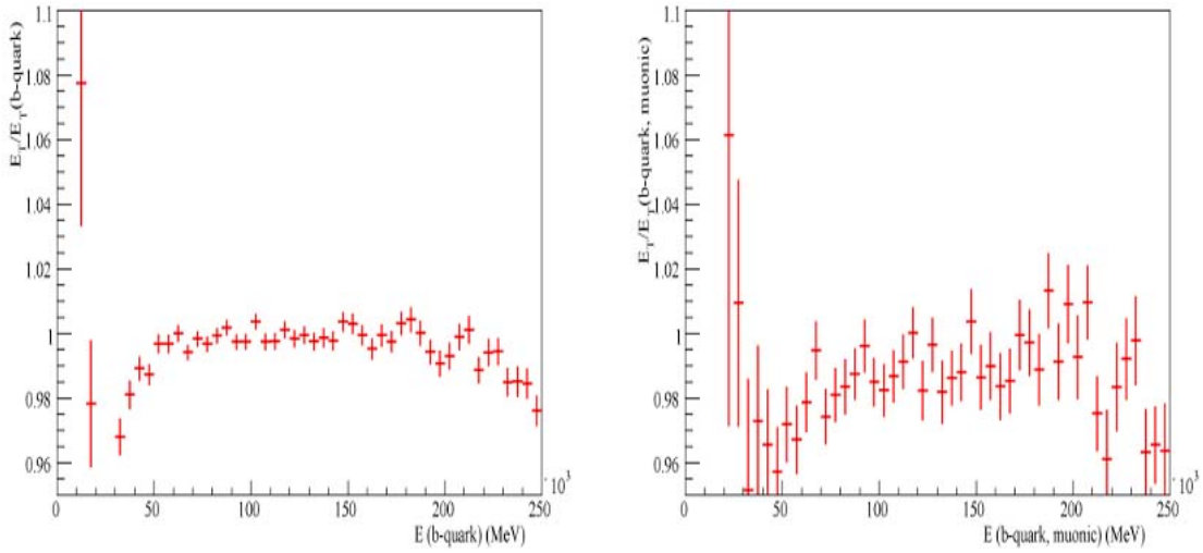
Figure 22: Check of the b -jet energy calibration.
