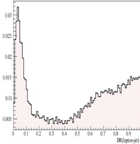
Figure 36: Distance between the leptons and the closest jet.
