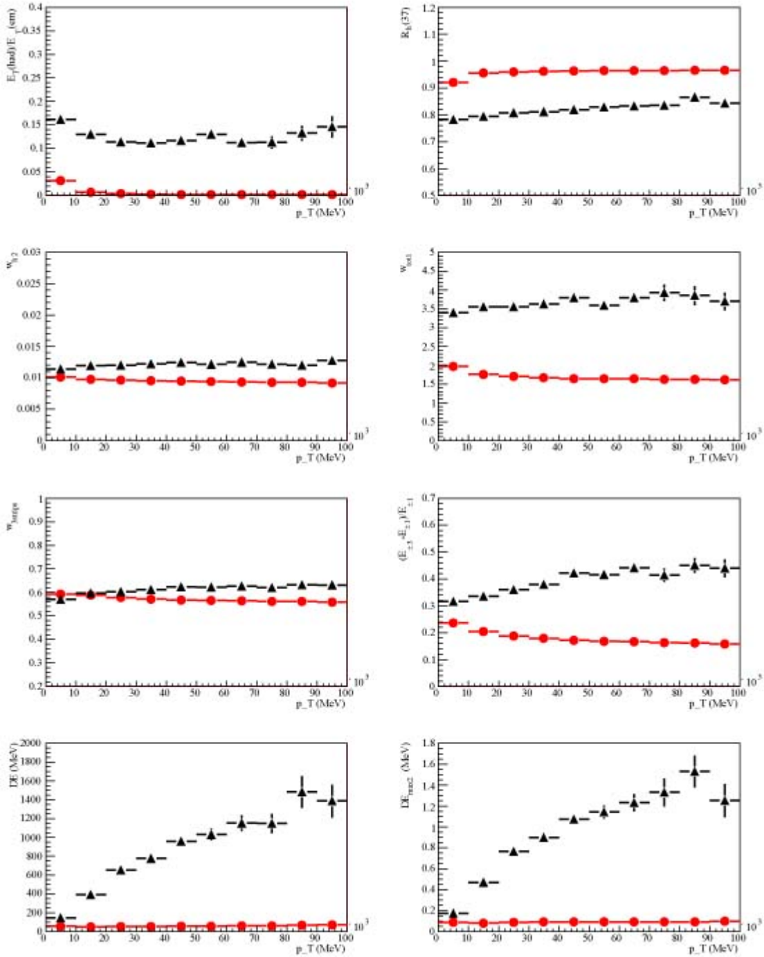
Figure 32: Distributions of the mean of each calorimetric discriminating variable as a function of the transverse momentum p_T for electrons (circle) and jets (triangle).
